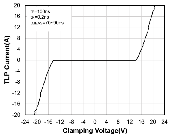
TLP Curve
